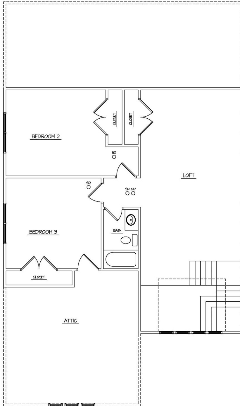
SECOND FLOOR PLAN B
